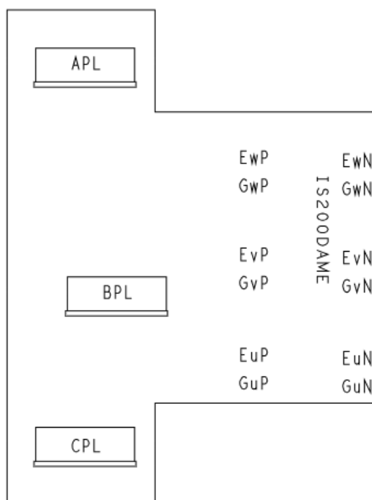
Figure 9. DAME Board Layout Diagram
