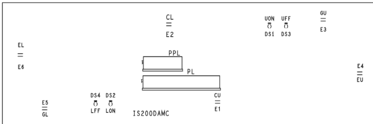
Figure 7. DAMC Board Layout Diagram
