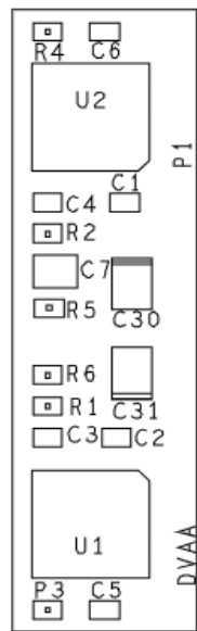
Figure 7. DVAA Daughterboard Layout Diagram
