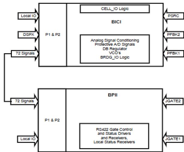
Figure 1. BICI Board and BP11 Board Interface Connections
