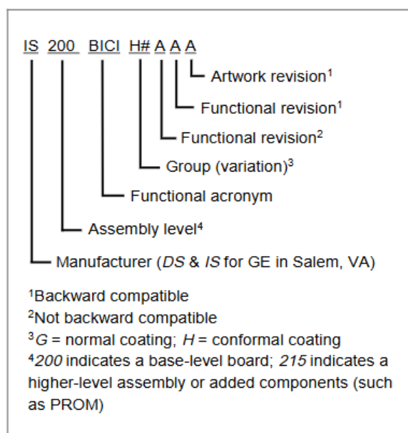
Figure 8. Board Part Number Conventions
