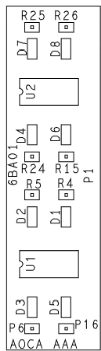
Figure 6. AOCA Daughterboard Layout Diagram
