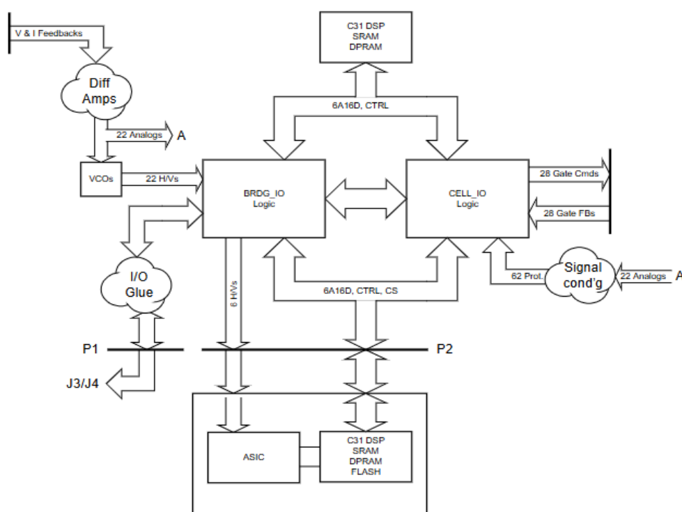
Figure 3. BICI Board Logic Architecture
