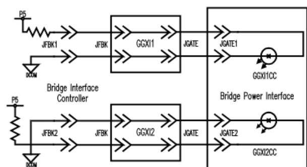
Figure 2. Board Identification Signals
